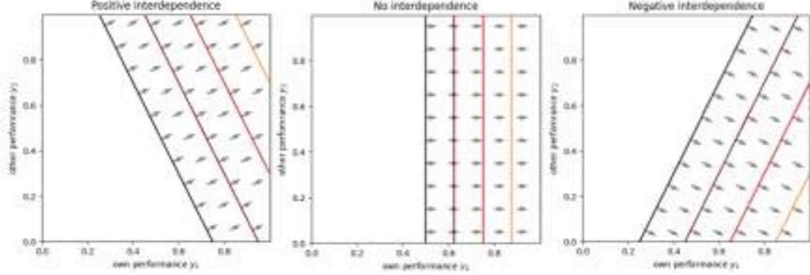
Figure 1. Isoquant maps of the \Psi metric and the corresponding gradient fields for different levels of \alpha . We consider three types of interdependencies, altruistic preferences \alpha = \frac{1}{2} (left panel), independent \alpha = 0 (middle) and adversarial \alpha = -\frac{1}{2} (right panel).
