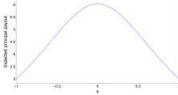
Figure 4. Expected payout by the principal as a function of \alpha in the example with the linear likelihood ratio and \theta = \frac{1}{2} .
