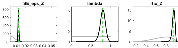
Figure 3: Prior and posterior distributions
